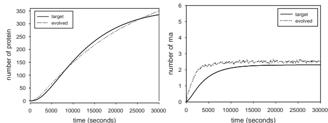
Figure 8: Target time series and the behaviour of the best model for positive autoregulation after changing the fitness function.
